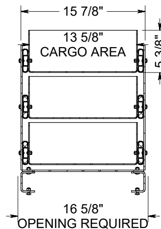
FRONT SECTION VIEW
