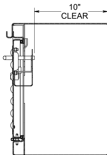
SIDE SECTION VIEW
