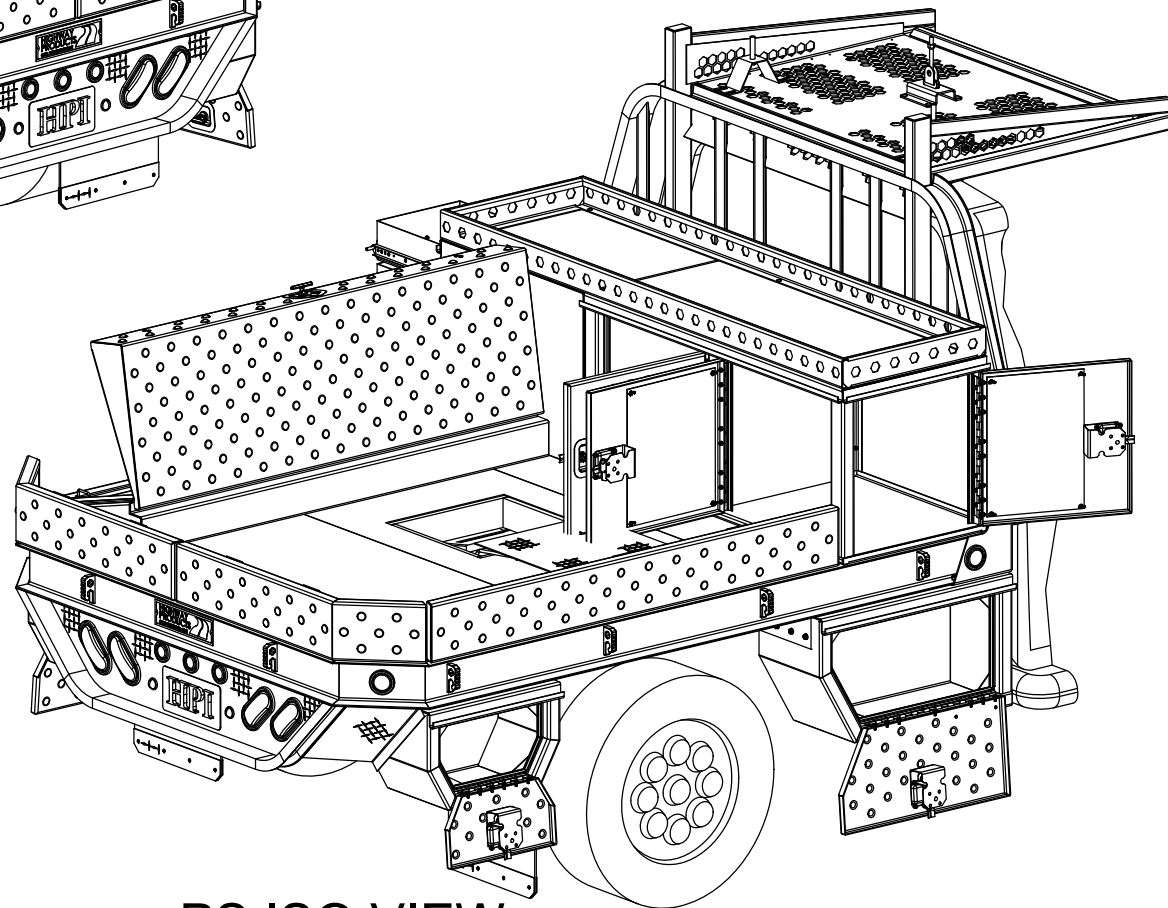
PS ISO VIEW
