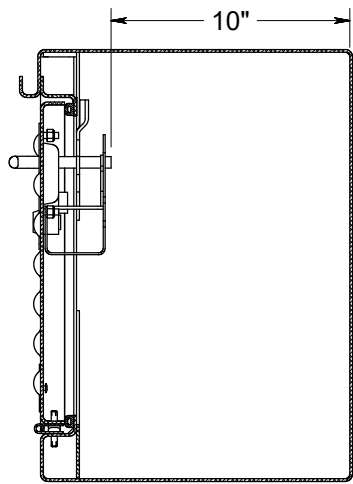
SIDE SECTION VIEW
