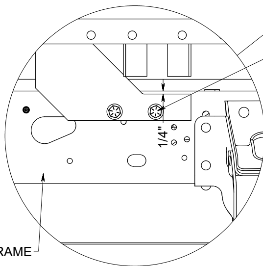
DETAIL K FRONT MOUNT FASTEN TO FRAME SCALE 1 : 8
