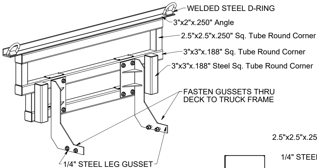
FRONT CAMPER MOUNT
