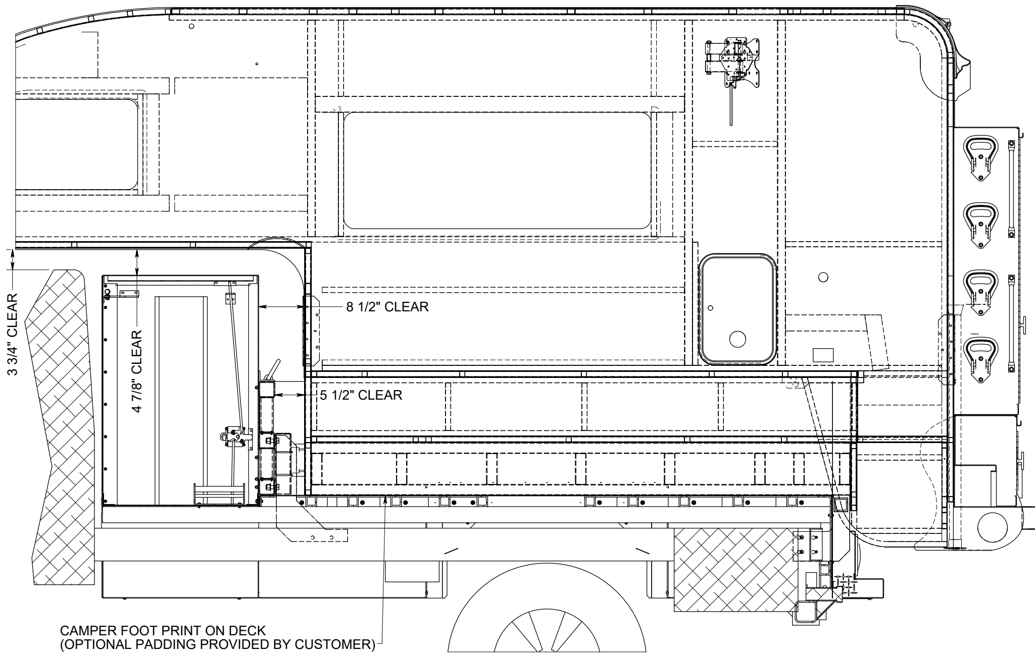
SIDE VIEW SECTION
