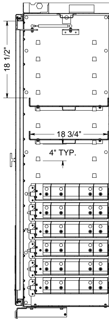
REAR SECTION
