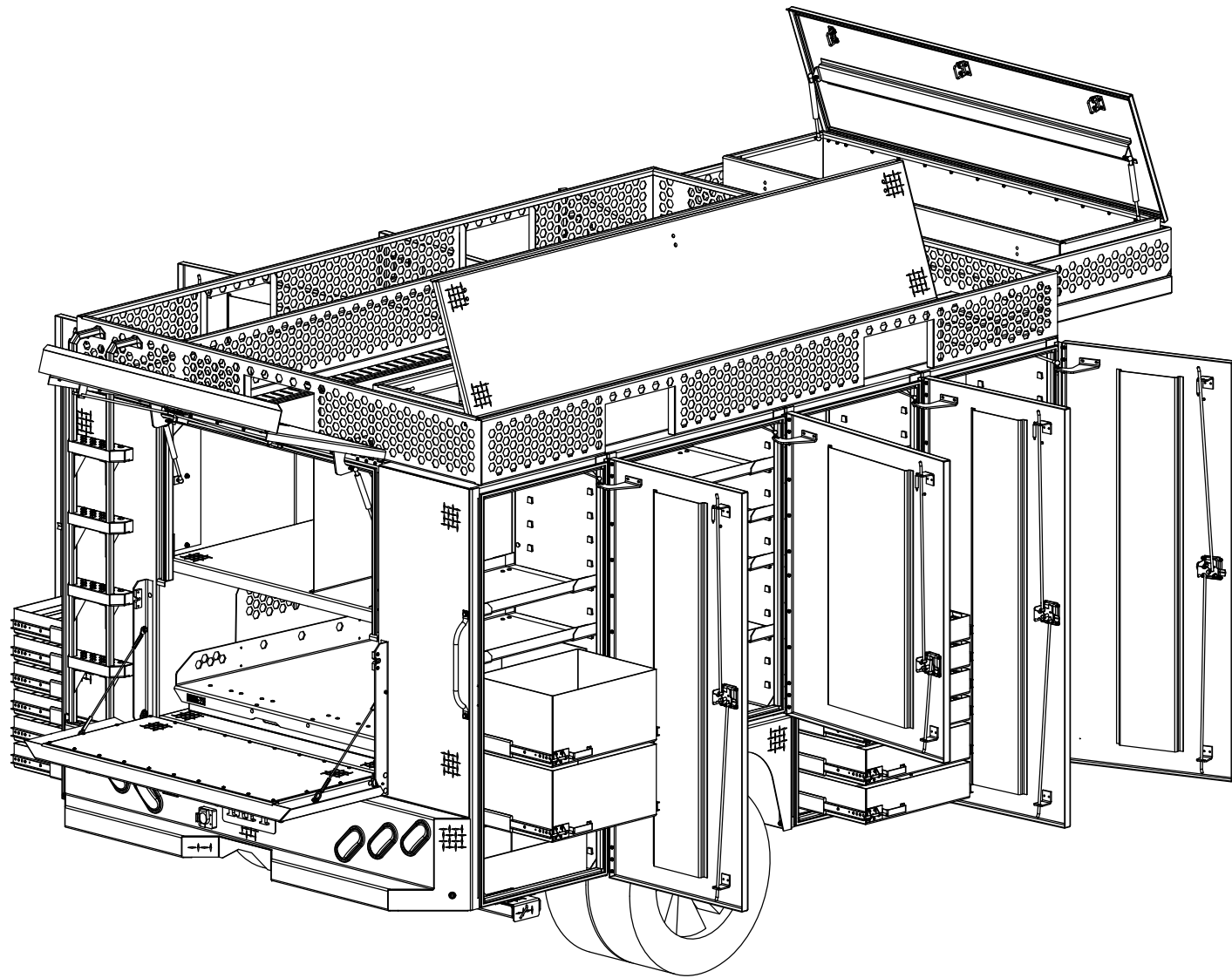
PS ISOMETRIC VIEW WITH THE DOORS OPEN
