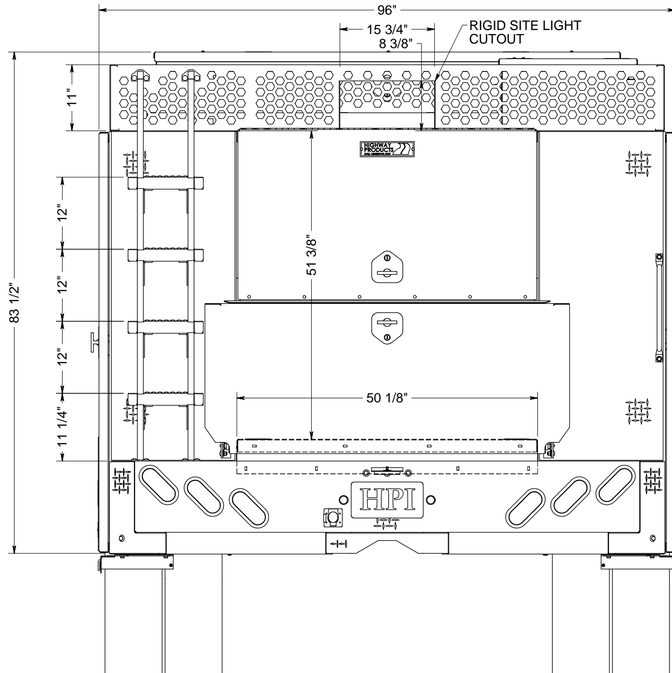
BACK VIEW
