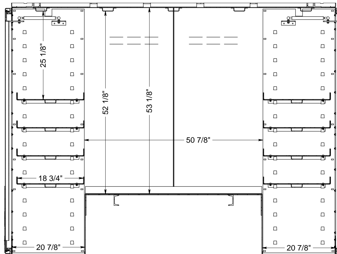
CROSS FRAME BOX SECTION VIEW
