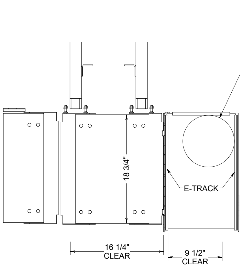
PS FRONT BOX TOP SECTION G-G SCALE 1 : 10
