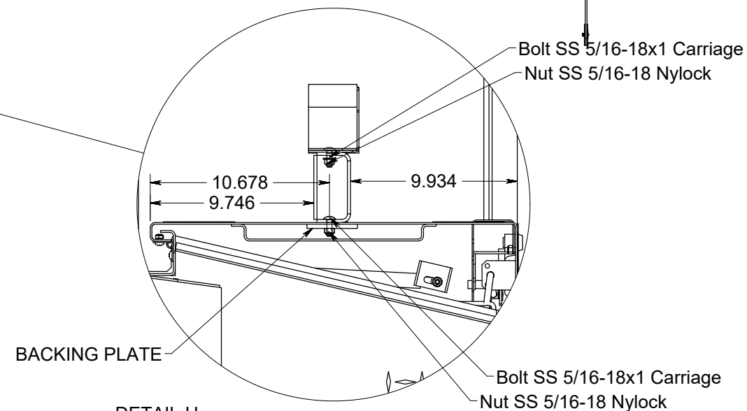
DETAIL H SCALE 1 : 8
