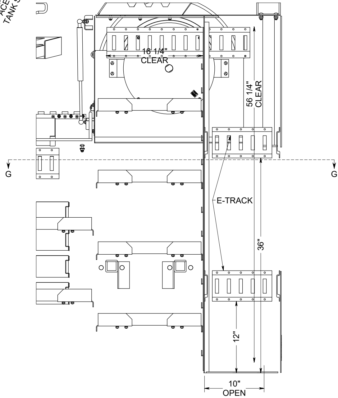
PS FRONT BOX DETAIL
