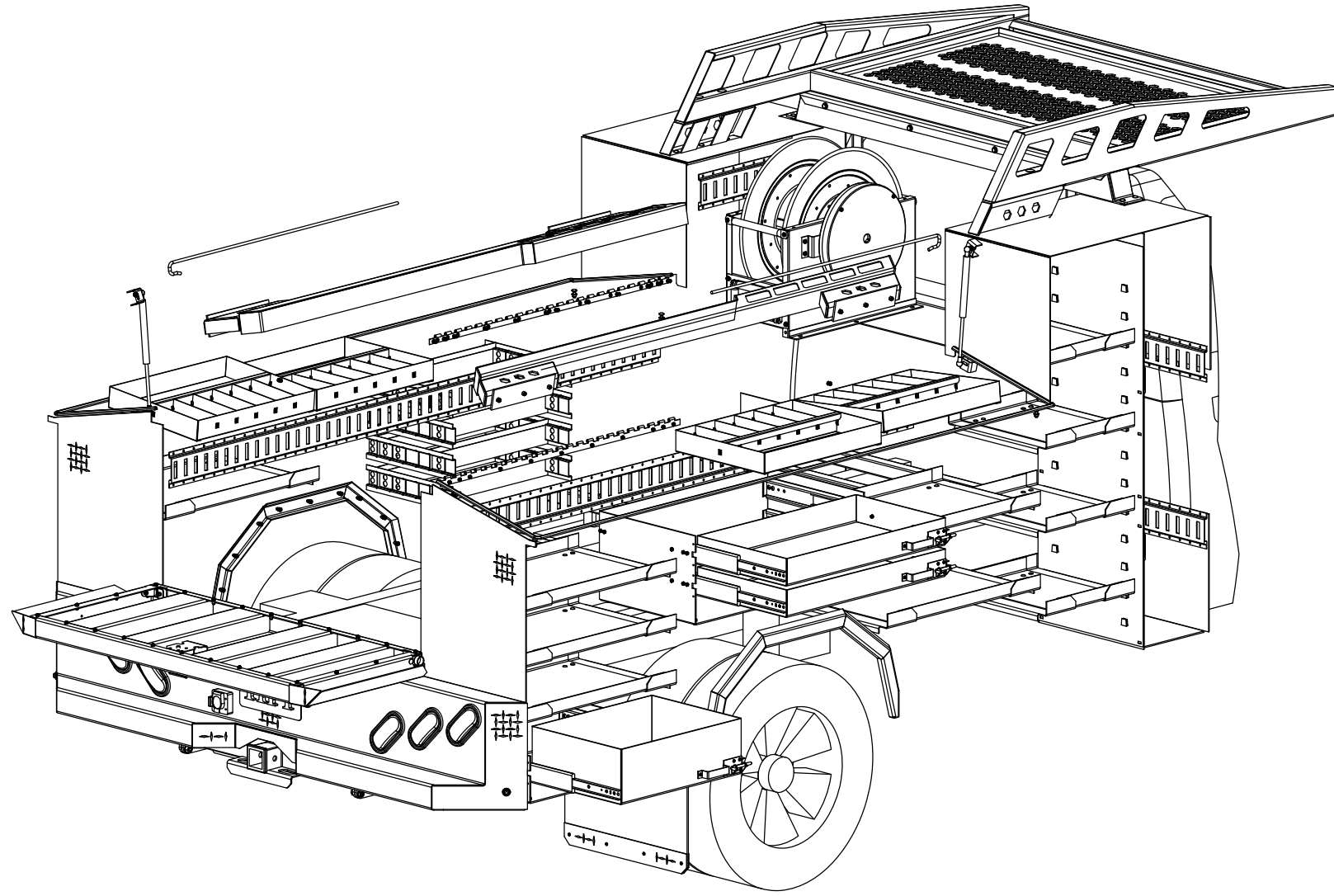
PS ISOMETRIC VIEW WITH THE DOORS OPEN
