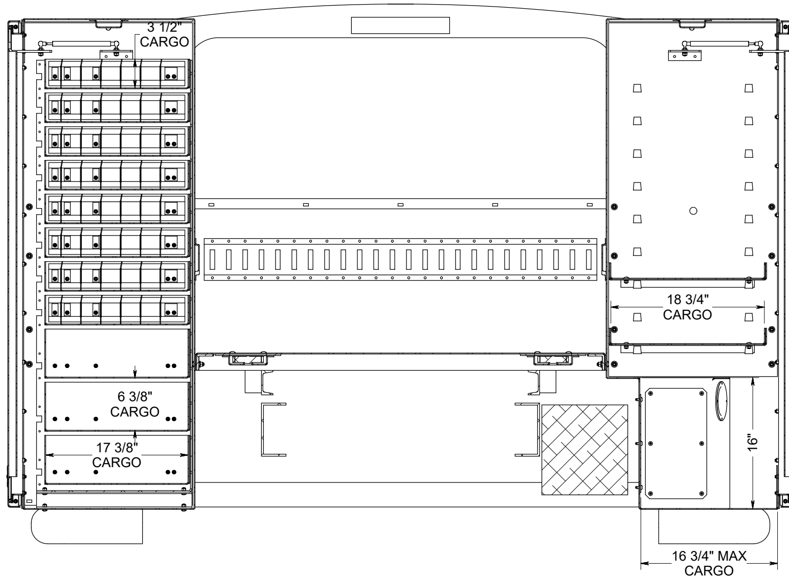
SECTION A-A FRONT SECTION VIEW
