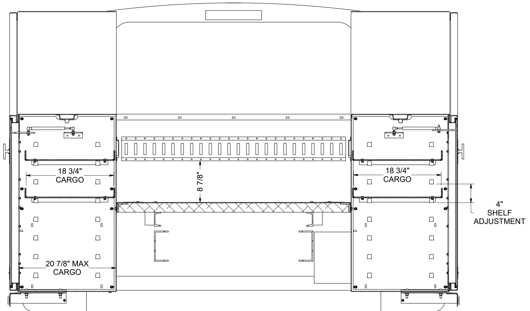
SECTION B-B SECOND BOX SECTION
