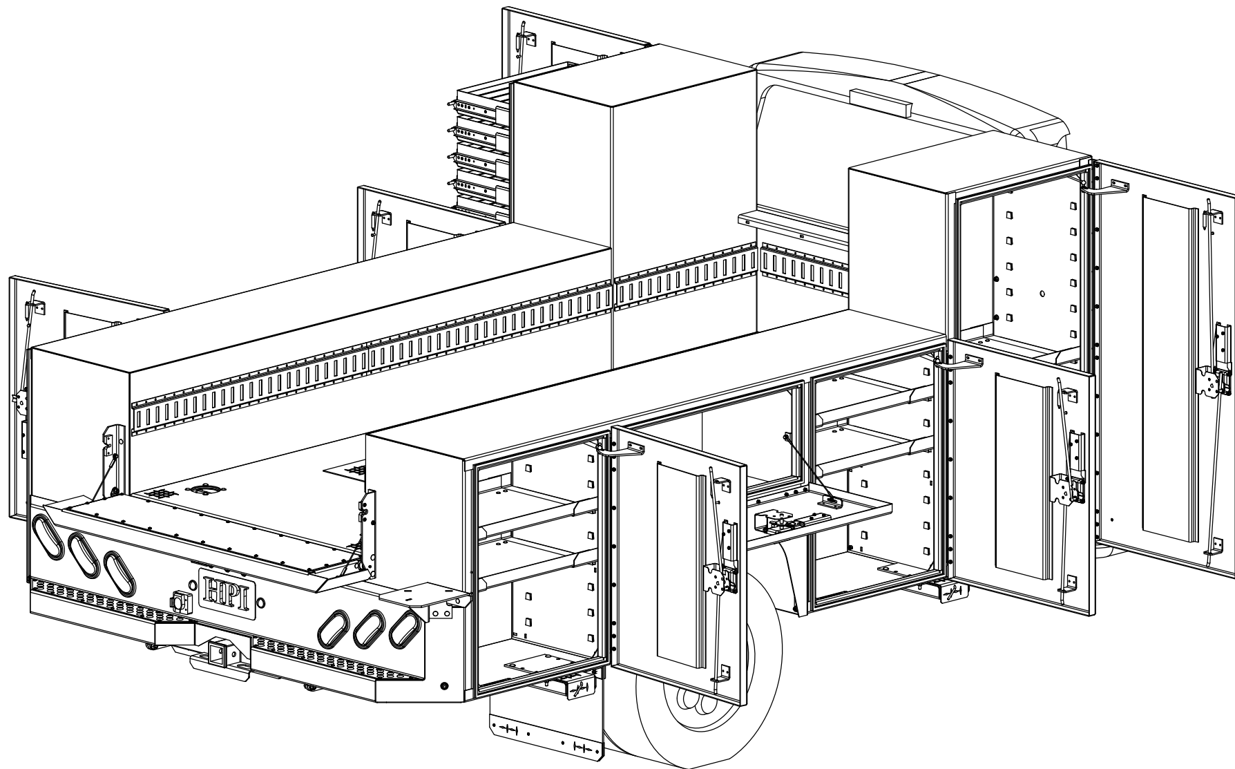
PS ISOMETRIC VIEW WITH THE DOORS OPEN
