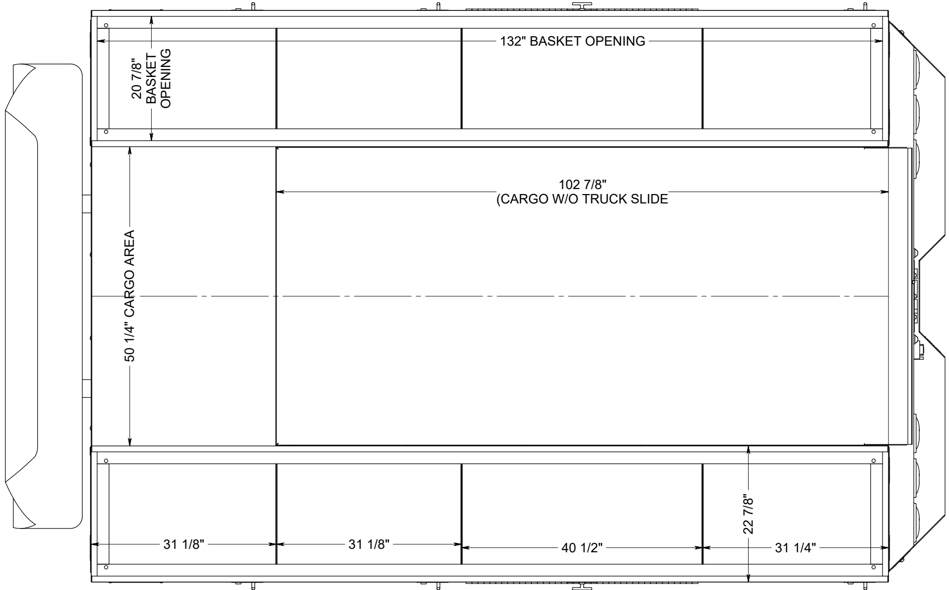
TOP VIEW
