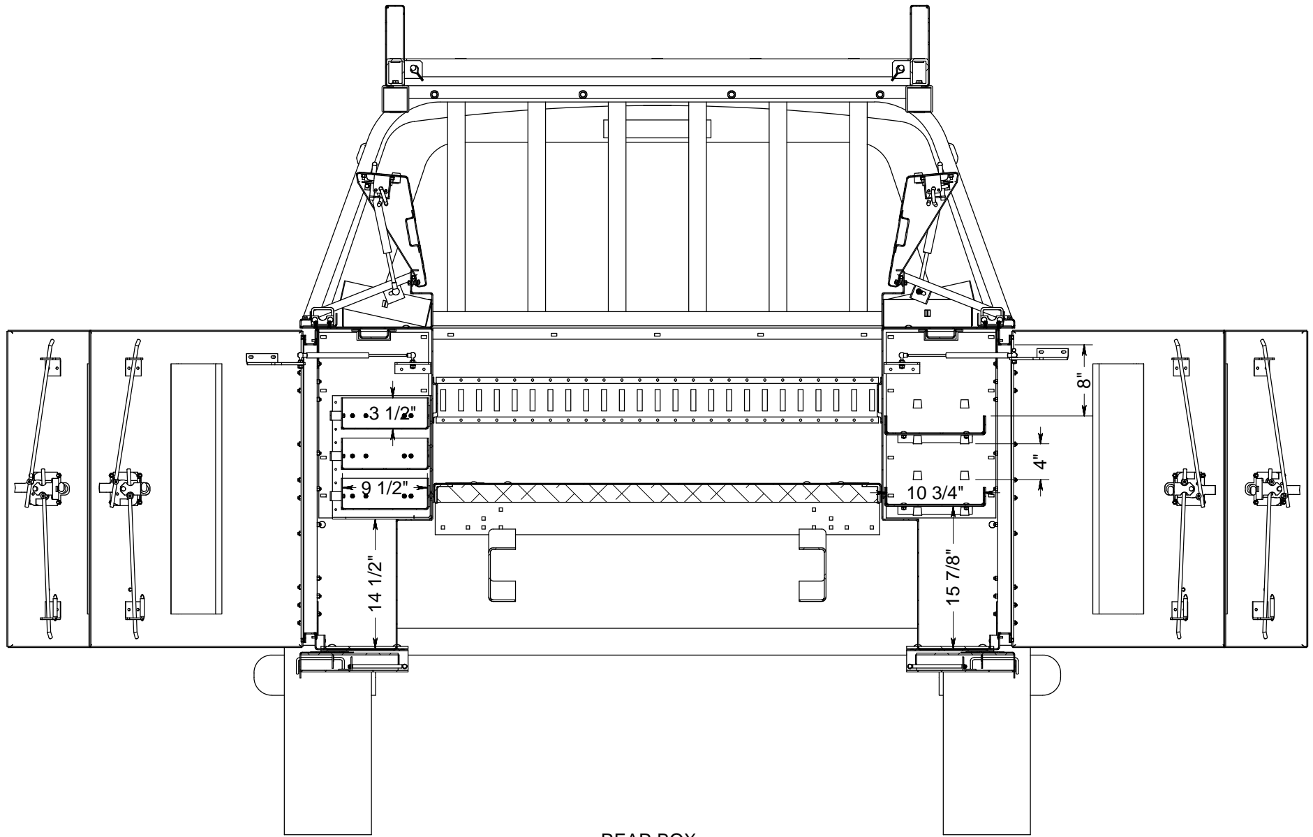
REAR BOX SECTION C-C
