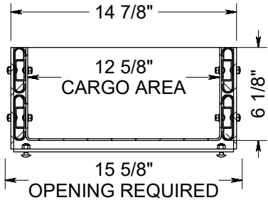
FRONT SECTION VIEW
